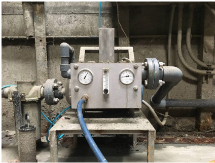
Picture 1: Moleaer XTB Nanobubble Generator installed at Chino plastics recycling plant.
