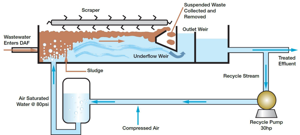
Figure 1: Conventional Dissolved Air Flotation (DAF) system
