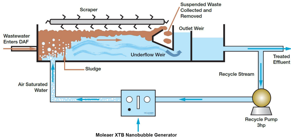
Figure 2: Moleaer XTB Nanobubble Generator installed in-line, utilizing a much lower HP-rated recirculating pump and eliminating the need for the pressurized tank.
